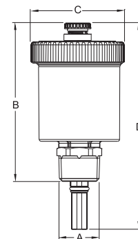
Model AVV-050 w/Service Check Valve
