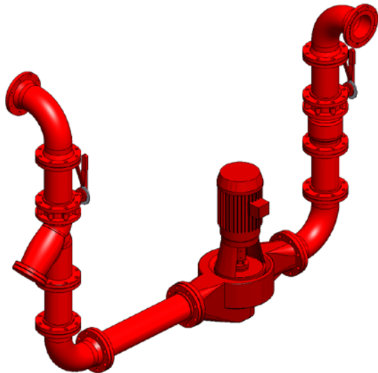
Implementing Split-coupled Vertical In-Line installation with traditional piping.
